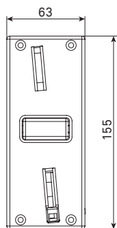
Gettoniera frontalino alto (per M10 e M20) High front plate for Coin Selector (for M10 and M20)
